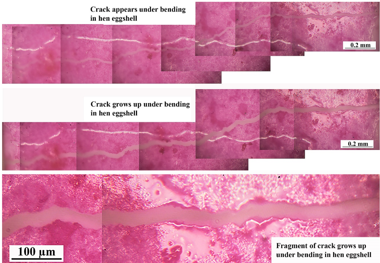
Fig. 16. Evolution of the crack in the sample of hen eggshell under bending in air: bending 1 (crack appearance); bending 2 (bending deflection is 100 \mu m).
