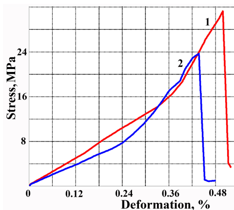
Fig. 4. Deformation curves of the samples cut from goose eggshell under bending in air: curve 1 – dry state; curve 2 – samples exposed to water for 24 hours.
