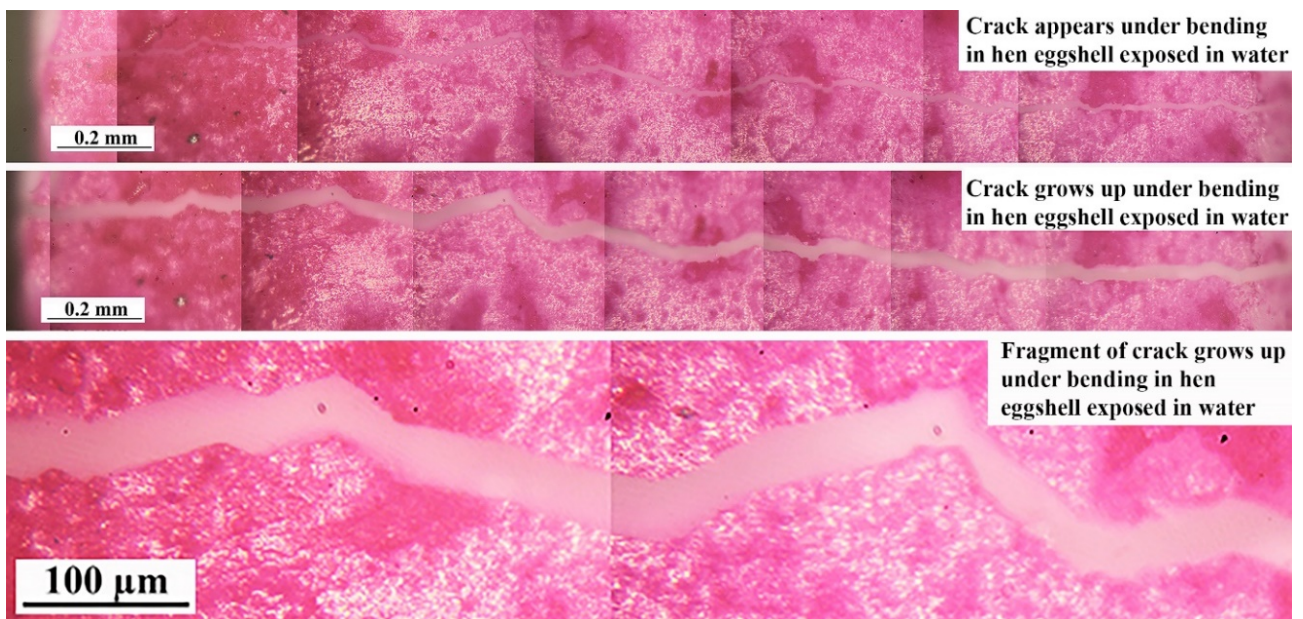
Fig. 17. Evolution of the crack in the sample of hen eggshell under bending in water: bending 1 (crack appearance); bending 2 (bending deflection is 50 \mu m).
